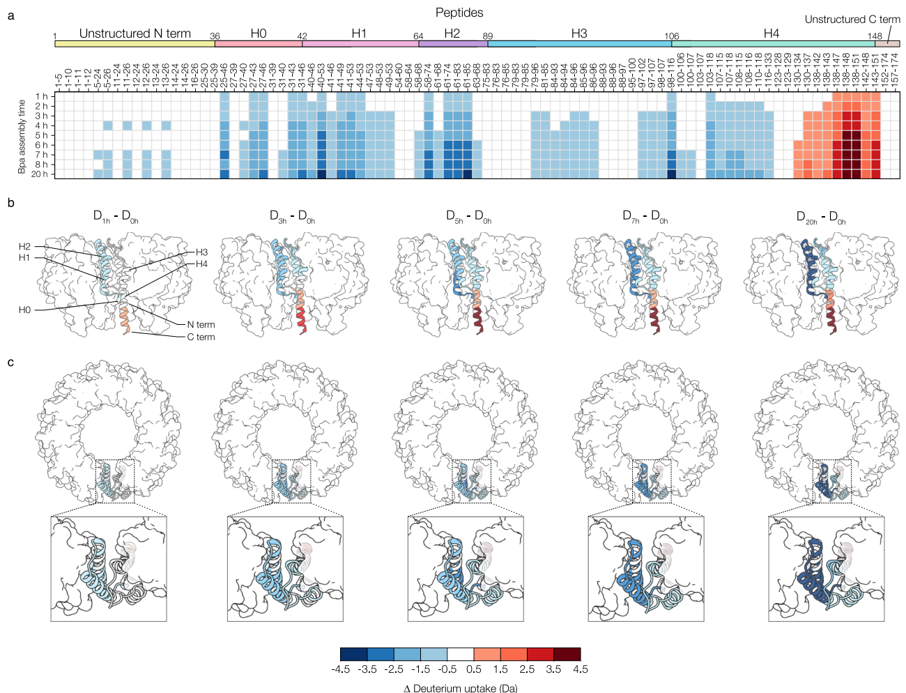
Fig. 2 | Pulsed HDX-MS reveals the time-dependent evolution of structure during dodecameric Bpa assembly. a Heatmap showing differential deuterium uptake following a 10-second D_2O pulse at various time points during Bpa assembly, relative to the onset of the assembly reaction ( t = 0 h). Bpa secondary structure elements and their corresponding residue numbers are denoted along the top of
