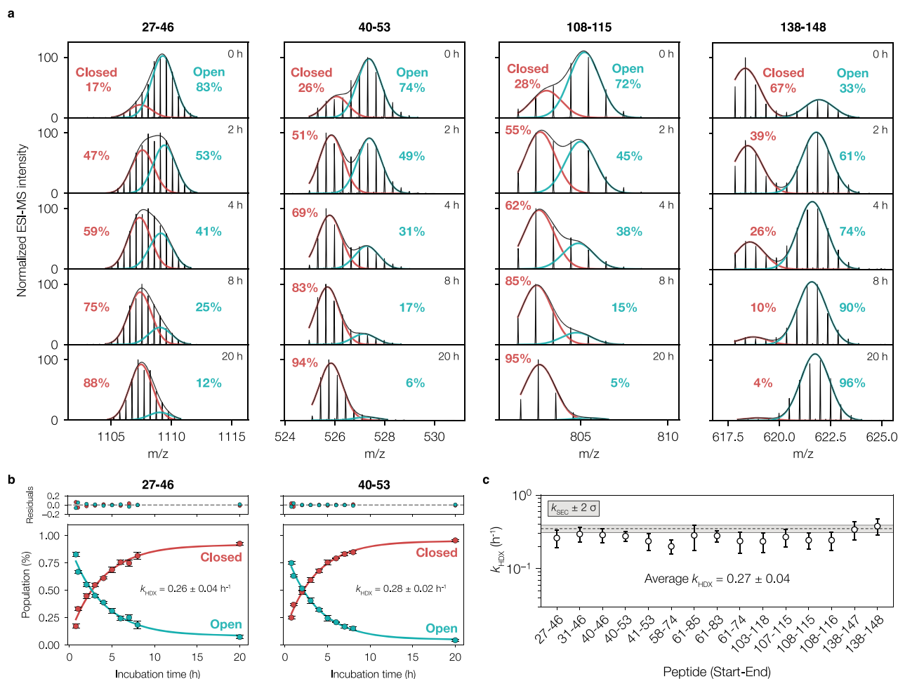
Fig. 3 | Bpa oligomerization interfaces exhibit asymmetric isotopic distributions during assembly, as revealed by pulsed HDX-MS. a A pair of Gaussian functions was fit to intensity profiles from peptides displaying asymmetric isotopic distributions and subsequently integrated. Closed (low HDX - red) and open (high HDX - teal) conformations and their fractional populations are denoted in the raw mass spectra. The displayed peptides are representative of others across the sequence but were selected to maximize sequence coverage; b Assembly time-dependent changes in the fractional populations of the open and closed conformations for two representative peptides were analyzed using a single-
