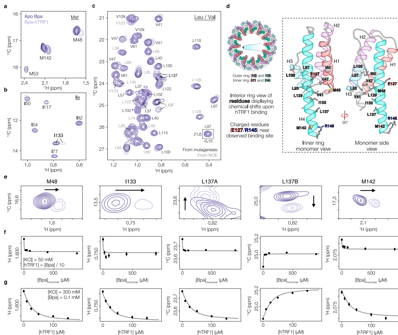
Fig. 5 | hTRF1 interacts with the C-terminal residues in the lower inner ring of dodecameric Bpa. Assigned a Met, b Ile, and c Leu/Val regions of a two-dimensional ^1\text{H} - ^{13}\text{C} HMQC spectrum for ILVM-labeled Bpa recorded at 40 °C and 18.8 T. Peaks depicted with dark purple contours are derived from apo Bpa and those with light purple contours from a complex of Bpa and [ ^2\text{H} ] hTRF1 in molar ratios of 100 \mu\text{M} (subunit concentration of Bpa): 150 \mu\text{M} (hTRF1) in the presence of 300 mM KCl; d Top view of the Bpa complex highlighting the inner and outer ring architecture. The inset shows a single Bpa subunit in cartoon representation, highlighting residues, shown as grey sticks, that display CSPs upon hTRF1 binding (PDB: 5LF) 13 . The sole charged residues proximal to these residues are shown in
