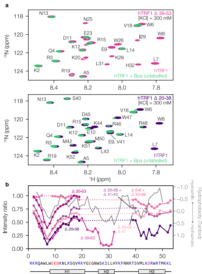
Fig. 6 | Hydrophobic patches and charged residues on hTRF1 mediate Bpa binding. a Superposition of ^1\text{H} - ^{15}\text{N} HSQC spectra of [ ^{15}\text{N} ]-labeled hTRF1 in the absence and presence of 10-fold monomer equivalents of unlabeled Bpa _{31-146} measured in the presence of 300 mM KCl, 40 °C. Top and bottom spectra were recorded on samples of hTRF1 \Delta_{39-53} and hTRF1 \Delta_{20-38} , respectively. b Intensity ratios for each hTRF1 peak in the absence and presence of unlabeled Bpa _{31-146} . The intensity ratios for each hTRF1 construct are colour-coded as indicated. The grey trace indicates the Tanford hydrophobic index 69 for the hTRF1 sequence. In the hTRF1 sequence, positively and negatively charged residues are denoted in blue and red, respectively.
