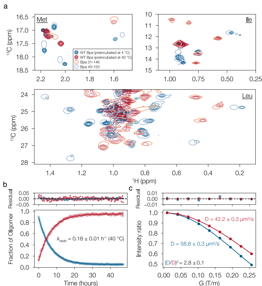
Fig. 4 | N- and C-terminal truncations stabilize specific oligomeric forms of Bpa. a ^1\text{H} - ^{13}\text{C} HMQC spectra for ILVM-labeled Bpa WT preincubated at 4 °C (multi-contour blue) or 40 °C (multi-contour red), Bpa 31-146 (single-contour red), and Bpa 45-153 (single-contour blue). All spectra were recorded at 40 °C and 18.8 T; b Changes in peak intensity for each oligomeric state (tetramer - blue, dodecamer - red) during a 48-hour acquisition. Data were fit assuming a first-order exponential model.
