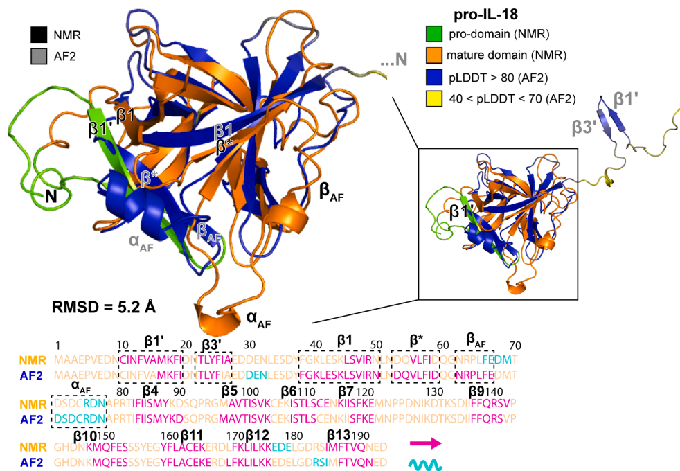
Fig. 1. Solution NMR structure of pro-IL-18 differs significantly from a high confidence predicted AF2 model. Overlay of the solution NMR structure of pro-IL-18 (pro-domain of pro-IL-18 in green, mature domain of pro-IL-18 in orange) and the AF2 prediction of this structure (yellow-blue gradient encoding predicted local-distance difference test (pLDDT) confidence values of 43–100). An RMSD value of 5.2 Å is calculated using backbone heavy atoms over the following residue ranges: 45–49 ( \beta 1 ), 55–58 ( \beta^* ), 82–88 ( \beta 4 ), 97–103 ( \beta 5 ), 107–113 ( \beta 6 ), 115–121 ( \beta 7 ), 137–142 ( \beta 9 ), 148–153 ( \beta 10 ), 159–165 ( \beta 11 ), 170–176 ( \beta 12 ), and 185–190 ( \beta 13 ), corresponding to the NMR-determined \beta strands from the mature domain of pro-IL-18 only [8]. These same atoms were used to align the two structures. Elements which are distinct between the NMR structure and AF2's prediction are labeled in black (NMR) and grey (AF2). \beta 3' in the NMR structure is not marked, as it is not visible in this view. However, it does hydrogen bond with \beta 1' as in the AF2 prediction. In addition, the locations of \alpha_{AF} and \beta_{AF} , as predicted by AF2, are displayed on the solution NMR structure (as well as on the AF2 model), and the position of \beta 1' (established experimentally) is indicated on the AF2 model. Beta strands (magenta) and alpha helices (cyan) are shown on the amino acid sequence, with significant differences between the NMR and predicted structures highlighted by the dashed boxes.
