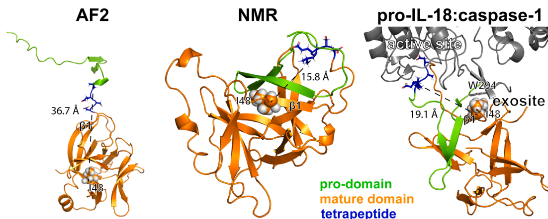
Fig. 4. AF2 predicted structure of pro-IL-18 is likely incompatible with caspase binding. Pro-IL-18 structures predicted by AF2 (left), determined by solution NMR (middle, PDB 8URV), and in complex with caspase-1 as established by cryo-EM (right, PDB 8SV1) are shown. The I48 sidechain is shown in spheres, while the tetrapeptide is shown in blue sticks. The sidechain of W294 from caspase-1 is shown in grey sticks. Dashed lines connect the C \alpha atoms of I48 (exosite) and L33 (tetrapeptide, active site), with the distance between these atoms noted. This distance is much larger in the AF2 predicted structure than in the complex with caspase-1, suggesting that the AF2 predicted structure would not be able to interact with both the active site and exosite of caspases-1/-4 simultaneously.
