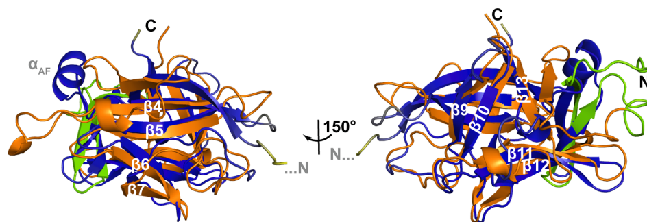
Fig. 2. C-terminal halves of solution NMR and AF2 predicted structures show significantly better agreement than N-termini. An overlay of the solution NMR structure of pro-IL-18 and the AF2 predicted model is displayed using the same color scheme as Fig. 1. Beta strands which are well-superimposed for the two structures are labeled in white. Beta strands \beta 4 - \beta 13 from the C-terminal half of the protein are labeled, and can be seen to be in reasonable agreement, in contrast to the structural elements in the N-terminal half highlighted in Fig. 1. While the backbone heavy atom RMSD of \beta 1 and \beta^* is 13.3 Å, the remaining \beta strands ( \beta 4 - \beta 13 ) have a backbone heavy atom RMSD of only 2.0 Å. If the structures are aligned using only \beta 4 - \beta 13 (see legend of Fig. 1 for residue ranges), this RMSD is reduced to 1.7 Å.
