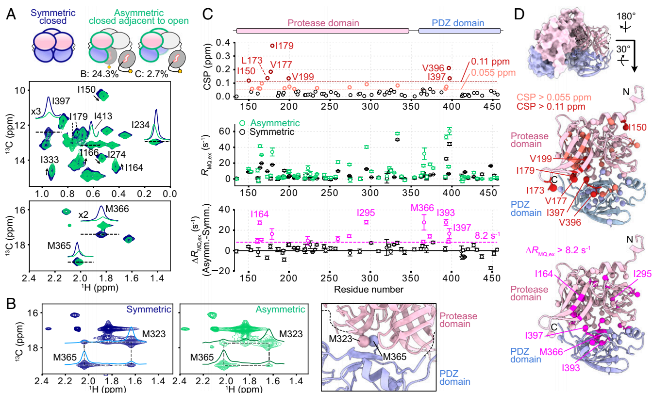
Fig. 3. Characterization of interprotomer allostery. (A) Superposition of 13 C- 1 H HMQC spectra of the symmetric U- 2 H, proR ILVM- 13 CH 3 S306A/I441V HtrA2 sample (navy) and the asymmetric HtrA2 sample prepared by mixing 90% U- 2 H, S306A/I441V/E425C PDZ-peptide-stapled/open protomers and 10% U- 2 H, proR ILVM- 13 CH 3 S306A/I441V protomers (green), focusing on the Ile (Top) and Met (Bottom) regions. The schematics for each sample are shown above the spectra. 1 H one-dimensional slices at the chemical shifts of the dotted lines are shown for I234, M365, M366, I397, and I413 in the same color as the two-dimensional contour. The slices for M366 and I397 are multiplied by factors of 2 and 3, respectively, for visualization. Methyl group assignments of the NMR closed protomer(s) of the asymmetric samples (green spectrum) were readily obtained from the assigned spectrum of the symmetric closed structure, as the chemical shift differences between the two spectra were small (<0.4 ppm, see C). The NMR datasets were recorded at 23.5 Tesla and 40 °C. (B) Selected regions of 1 H- 13 C [ t 1 ]- t mix - 1 H [ t 2 ] NOESY spectra of the symmetric (Left) and asymmetric (Right) samples are shown (200 ms mixing time). Cross- and diagonal-peaks for M323 and M365 are connected with dotted boxes to aid in visualization. (Right Inset) A portion of the HtrA2 protomer structure (PDB ID: 1LCY) is shown, with the C \epsilon carbons of M323 and M365 denoted as spheres. NMR datasets were recorded at 14.0 Tesla and 40 °C. (C, Top) Plot of CSP values between symmetric and asymmetric samples, 23.5 Tesla 40 °C. Methyl groups with CSPs larger than one (light orange) or two (dark red) SD (>0.055 and 0.11 ppm, respectively) are indicated. CSP values for each type of methyl-bearing residue were calculated as \Delta\delta = \sqrt{(\Delta\delta_H/\alpha)^2 + (\Delta\delta_C/\beta)^2} , where \Delta\delta_H and \Delta\delta_C are the chemical shift differences in the 1 H and 13 C dimensions, and \alpha and \beta are the SDs of the 1 H and 13 C chemical shift distributions deposited in the Biological Magnetic Resonance Data Bank ( \alpha = 0.282 , \beta = 1.646 for Ile; \alpha = 0.273 , \beta = 1.582 for Leu; \alpha = 0.259 , \beta = 1.358 for Val; \alpha = 0.387 , \beta = 1.736 for Met). (Middle) Plot of the exchange contributions to 13 C- 1 H MQ relaxation rates ( R MQ,ex ) for the symmetric (black circle) and asymmetric (green circle) HtrA2 samples at 14.0 Tesla. (Bottom) Plot of the difference in R MQ,ex values between symmetric and asymmetric samples ( \Delta R_{MQ,ex} ) calculated as \Delta R_{MQ,ex} = R_{MQ,ex}[\text{asymmetric}] - R_{MQ,ex}[\text{symmetric}] . \Delta R_{MQ,ex} values larger than one SD (>8.2 s -1 ) are colored in magenta, and those larger than two SD (>16.4 s -1 ) are labeled by methyl residue. (D) proR ILVM-methyl groups from C with significant CSPs (>1 SD) (Top, light orange and deep red spheres) and \Delta R_{MQ,ex} values (Bottom, magenta spheres) mapped onto the HtrA2 protomer (PDB ID: 1LCY). Effective concentrations of NMR-active protomers in particles B and C were 20 and 4.5 \mu\text{M} , respectively.
