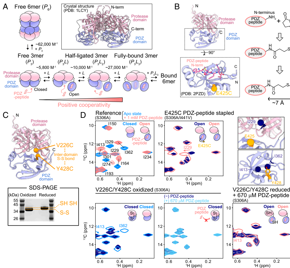
Fig. 1. Controlling domain opening via Cys-based chemistry. (A) The oligomerization and PDZ-peptide binding mechanism of HtrA2, as established in our previous study (26). (Inset) Crystal structure of trimeric HtrA2 (PDB ID: 1LCY). The protease (residues 134 to 345) and PDZ (residues 359 to 458) domains are colored pink and light blue, respectively. Electron density for residues 282 to 290 ( \beta 8- \beta 9 linker) and 344 to 358 (interdomain linker) is not observed; these regions are shown with dotted lines. (B) The crystal structure of the isolated PDZ domain of HtrA2 in complex with peptide (WTMFVW; PDB ID: 2PZD). The peptide is shown as a pink stick model with the E425 C \beta carbon displayed as an orange sphere. Chemical structures of the components involved in the Cys modification approach to control the peptide-bound state of the PDZ domain are shown on Right. (C, Top) The C \beta carbons of V226 and Y428 are displayed on an HtrA2 protomer (PDB ID: 1LCY). (Bottom) SDS-PAGE analysis of V226C/Y428C/S306A HtrA2 under oxidizing and reducing conditions. (D, Left Top) ^{13}\text{C} - ^1\text{H} HMQC spectra of U- ^2\text{H} , proR ILVM S306A HtrA2 in the absence (blue) and presence (pink) of 1 mM PDZ-peptide. (Center Top) ^{13}\text{C} - ^1\text{H} HMQC spectrum of U- ^2\text{H} , proR ILVM S306A/I441V/E425C PDZ-peptide-stapled HtrA2 (navy). The spectrum of U- ^2\text{H} , ILVM S306A/I441V HtrA2 in the presence of 1 mM PDZ-peptide is shown using pink single contours. (Left Bottom) ^{13}\text{C} - ^1\text{H} HMQC spectrum of U- ^2\text{H} , proR ILVM V226C/Y428C/S306A HtrA2 under oxidizing conditions. The spectrum of U- ^2\text{H} , proR ILVM S306A HtrA2 is shown with single blue contours. (Center Bottom) Superposition of ^{13}\text{C} - ^1\text{H} HMQC spectra of U- ^2\text{H} , proR ILVM V226C/Y428C/S306A HtrA2 in the absence (navy) and presence of 670 \mu\text{M} PDZ-peptide (cyan) under oxidizing conditions. (Right Bottom) ^{13}\text{C} - ^1\text{H} HMQC spectrum of U- ^2\text{H} , proR ILVM V226C/Y428C/S306A HtrA2, fully reduced and in the presence of 670 \mu\text{M} PDZ-peptide (navy). The spectrum of U- ^2\text{H} , proR ILVM S306A HtrA2 in the presence of 1 mM PDZ-peptide is shown with pink single contours. Schematics of the protomeric structures that form the HtrA2 trimers studied by NMR are shown in the upper right hand corner of each spectrum. (Right Top) The methyl groups with significant chemical shift differences in the comparative spectra shown (i.e., between Cys and Cys-less molecules) (navy spheres) are in the immediate vicinity of the mutated residues (C \beta carbon of E425 shown as an orange sphere and side-chain atoms of Y428 shown as orange sticks) (PDB ID: 1LCY). Methyl group assignments of the S-S-locked and PDZ-peptide-stapled samples were obtained by inspection of spectra of the closed and open structures, respectively, as there were only minor chemical shift differences. All NMR data were recorded at 23.5 Tesla and 40 ^{\circ}\text{C} .
