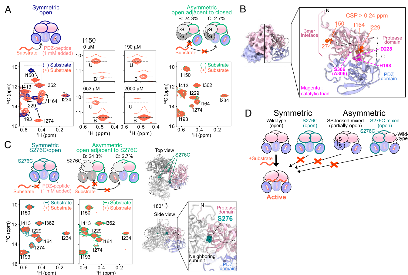
Fig. 5. Interprotomer allostery regulates formation of the active conformation. (A, Left) Superposition of ^{13}\text{C} - ^1\text{H} HMQC spectra of the symmetric U\text{-}^2\text{H} , proR ILVM- ^{13}\text{CH}_3 S306A/I441V HtrA2 sample (100 \mu\text{M} ), 1 mM PDZ-peptide, in the absence (navy) and presence (orange) of 2 mM substrate (20-fold excess over HtrA2 protomers). (Center) Selected region of HMQC datasets recorded at four different concentrations of substrate (0, 190, 653, and 2,000 \mu\text{M} ) and focusing on I150, located at the interprotomer domain interface (see B). (Right) Superposition of ^{13}\text{C} - ^1\text{H} HMQC spectra of the asymmetric HtrA2 sample (150 \mu\text{M} ), prepared by mixing 90% U\text{-}^2\text{H} , Met- ^{13}\text{CH}_3 V226C/Y428C/S306A/I441V S-S-locked/closed protomers and 10% U\text{-}^2\text{H} , proR ILV- ^{13}\text{CH}_3 S306A/I441V protomers, 1 mM PDZ-peptide, in the absence (light green) and presence (orange) of 2 mM substrate. The schematics for each type of sample are shown on top of the spectra. (B) Ile methyl groups with significant CSPs ( >1\text{ SD} = 0.24\text{ ppm} ) upon substrate binding are mapped onto an HtrA2 protomer (PDB ID: 1LCY) in orange, with remaining Ile methyl carbons highlighted as spheres. The residues forming the catalytic triad, H198, D228, and S306 (Ala in the structure), are shown as magenta sticks. CSPs were calculated as described in the legend to Fig. 3C. (C, Left) Superposition of ^{13}\text{C} - ^1\text{H} HMQC spectra of the symmetric U\text{-}^2\text{H} , ILVM- ^{13}\text{CH}_3 S276C/S306A/I441V HtrA2 sample in the absence (light green) and presence (orange) of 2 mM substrate. (Right) Superposition of ^{13}\text{C} - ^1\text{H} HMQC spectra of the asymmetric HtrA2 sample prepared by mixing 90% U\text{-}^2\text{H} , S276C/S306A/I441V protomers and 10% U\text{-}^2\text{H} , proR ILVM- ^{13}\text{CH}_3 S306A/I441V protomers in the absence (light green) and presence (orange) of 2 mM substrate. Schematics for each type of sample are shown above the spectra. (Right Inset) S276 atoms are shown as spheres in the HtrA2 trimer structure (PDB ID: 1LCY). The neighboring subunit is colored in gray for visualization. (D) Schematic summarizing the NMR experiments shown in A and C. All NMR data sets were recorded at 23.5 Tesla and 40 °C in the presence of 200 mM NaCl.
