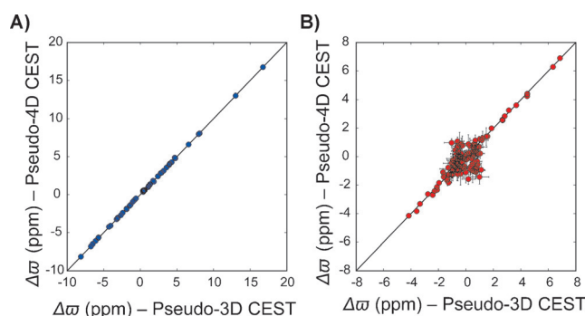
Figure 3. Linear correlation plots of \Delta\tilde{\omega} values extracted from uniformly sampled, Fourier transformed pseudo-3D CEST (X-axis) and from non-uniformly sampled pseudo 4D HNCO-based CEST (Y-axis) experiments for A) G48A Fyn SH3 and B) L99A T4L. Error bars smaller than the size of the symbols are not displayed.
