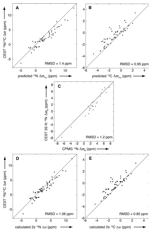
Figure 3. A39G FF folds via an intermediate state, as detected by ^{15}\text{N} - and ^{13}\text{C} -CEST experiments. Comparison of predicted ^{15}\text{N} (A) and ^{13}\text{C} (B) \Delta\varpi values assuming an unfolding transition ( \Delta\varpi_{\text{FU}} , x axis) with those obtained via CEST ( \text{CEST } \Delta\varpi , y axis) measured on a [U- ^{15}\text{N} , ^{13}\text{C} ] sample of A39G FF, 1 °C. A two-site exchange model has been assumed. C) Correlation between \varpi_{\text{I}} values from fits of CEST profiles to a 3-site exchange model (FIU, A39G FF, y axis) and intermediate chemical shifts from analysis of CPMG data recorded on the WT FF domain (x axis). D,E) The systematic deviations in (A,B) are reduced by taking into account the I state chemical shifts, as described in the text.
