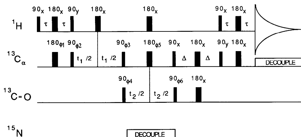
FIG. 3. Pulse sequence for the HCACO experiment. Typical delay durations are \tau = 1.5 ms and \Delta = 3 ms. The power levels of the \text{C}_\alpha and \text{C}' pulses are adjusted such that during application of a \text{C}_\alpha pulse minimal \text{C}' excitation occurs, and vice versa. On a 500 MHz spectrometer, for a 120 ppm difference of the \text{C}' and \text{C}_\alpha carrier positions, this condition may be achieved by adjusting the RF field strengths to 3.9/N kHz ( N = 1, 2, \dots ). In order to minimize the effects of homonuclear J modulation by the passive \text{C}_\alpha – \text{C}_\beta couplings during the intervals \Delta , the RF field strength of the 180_x ( \text{C}_\alpha ) pulse may be reduced to 1.95 kHz. Note that because a change in power frequently also introduces a phase shift, it may be necessary to use the same low power level for the two 90_x and 90_y \text{C}_\alpha pulses immediately preceding and following the \Delta intervals. The phase cycling employed is as follows: \phi_1 = x, -x ; \phi_2 = x ; \phi_3 = y, -y ; \phi_4 = 2(x), 2(-x) ; \phi_5 = 4(-x) ; \phi_6 = 8(x), 8(-x) ; Acq. = 2(x, -x, -x, x), 2(-x, x, x, -x) . The phases \phi_2 and \phi_4 are incremented by 90^\circ to generate complex data in the t_1 and t_2 dimensions respectively.
