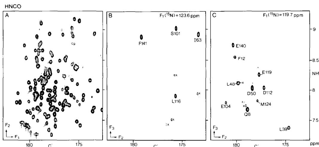
FIG. 6. (A) Section of the 2D NH-C' correlation spectrum of calmodulin, recorded with the pulse scheme of Fig. 1 but leaving the t_1 evolution time in this pulse scheme fixed at 2 \mu s. Apart from higher digital resolution in the C' dimension, this 2D spectrum corresponds to the projection onto the ( F_2 , F_3 ) plane of the 3D HNCO spectrum. Correlations for side chains of Asn and Gln residues are marked by arrows. (B, C) Sections from ( F_2 , F_3 ) slices of the HNCO 3D spectrum, taken at F_1 ( ^{15}\text{N} ) chemical shifts of 123.6 and 119.7 ppm. The 3D spectrum results from a (32 complex) \times (64 complex) \times (512 real) data matrix (4 Mword), with acquisition times of 30 ( t_1 ), 46 ( t_2 ), and 64 ( t_3 ) ms. After zero filling the digital resolution is 17 ( F_1 , ^{15}\text{N} ), 5.4 ( F_2 , C'), and 8 Hz ( F_3 , NH). The 16-step phase cycle was repeated four times to obtain complex data in both the t_1 and the t_2 dimensions, resulting in 128 scans per hypercomplex ( t_1 , t_2 ) pair. Using a 1.16 s delay between scans, the total measuring time was 46 h. The delay \tau was 1.5 ms, and \delta was set to 18 ms. Baseline correction in the t_3 dimension of the time-domain data was used to reduce the intensity of the residual H 2 O signal (40); no frequency-domain baseline correction or any other cosmetic procedures were used. Weak resonances due to proteolytic degradation and partial ( \sim 15\% ) deamidation of Gln and Asn residues are marked x. Resonances from proteolytic cleavage products are easily recognized because their intensity increases with the age of the sample.
