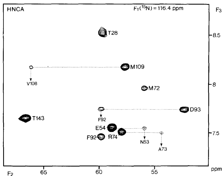
FIG. 7. Part of an ( F_2 F_3 ) slice of the HNCA 3D spectrum, taken at an F_1 ( ^{15}\text{N} ) chemical shift of 116.4 ppm, displaying intense intraresidue NH- \text{C}\alpha correlations and weaker correlations between NH and the \text{C}\alpha resonance of its preceding residue. The 3D spectrum results from a (32 complex) \times (64 complex) \times (512 real) data matrix (4 Mword), with acquisition times of 30 ( t_1 ), 14.8 ( t_2 ), and 64 ( t_3 ) ms. After zero filling, the digital resolution is 17 ( F_1 , ^{15}\text{N} ), 17 ( F_2 , \text{C}\alpha ), and 8 Hz ( F_3 , NH). The total measuring time was 43 h. The delay \tau was 1.5 ms and \delta was set to 33 ms. No baseline correction was used during data processing.
