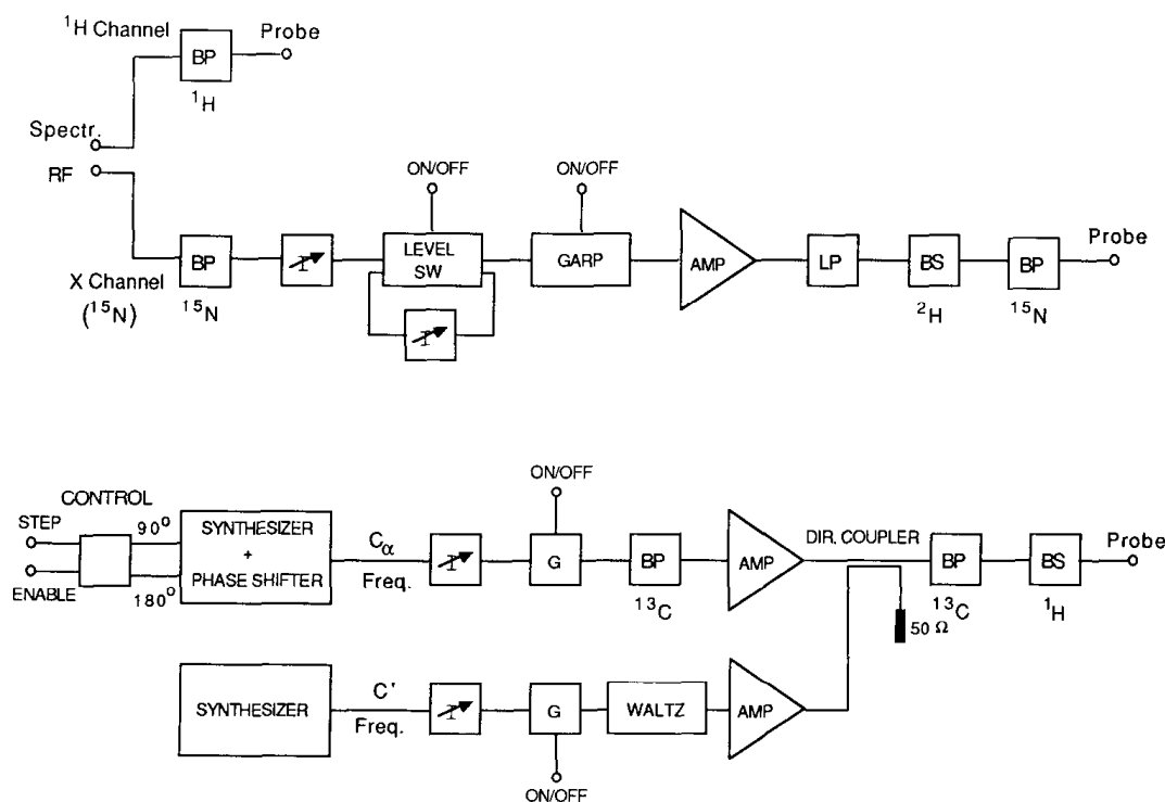
FIG. 5. Hardware configuration for the HNCA experiment. The bandpass filters (BP), RF gates (G), GARP and WALTZ modulators, and band-stop filters (BS), as well as the directional coupler (terminated by 50\ \Omega ) are all homebuilt. All amplifiers (AMP) are of the class A type with a maximum output power of 20 W. The RF gates each use two fast RF switches (DOTY Electronics) and in the off-mode provide more than 70 dB attenuation.
