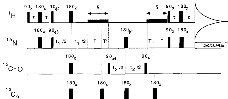
FIG. 1. Pulse scheme of the HNCO experiment. Typical delay durations used in this experiment are \tau = 2.25 \text{ ms} , \delta = 18 \text{ ms} , T = 14 \text{ ms} , and T' = 4 \text{ ms} . Presaturation of the \text{H}_2\text{O} resonance (not shown) is needed when the experiment is recorded in \text{H}_2\text{O} solution. In addition, water saturation is employed during both \delta periods. The phase cycling used is as follows: \phi_1 = x, -x ; \phi_2 = y, -y ; \phi_3 = x ; \phi_4 = 2(x), 2(-x) ; \phi_5 = 4(x), 4(y), 4(-x), 4(-y) ; Acq. = x, 2(-x), x, -x, 2(x), -x . The phases \phi_3 and \phi_4 are independently incremented by 90^\circ to generate complex data in the t_1 and t_2 dimensions, respectively. In both the t_1 and t_2 dimensions, quadrature detection is achieved using the TPPI–States method (34).
