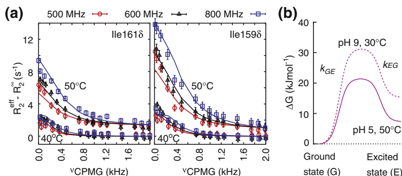
Fig. 3. The motions of I159 and I161 are critical for the control of quaternary dynamics. (a) 13 C δ1 CPMG relaxation dispersion profiles of I159/I161 measuring effective transverse relaxation rates ( R_2^{\text{eff}} ) as a function of the strength of an applied radiofrequency field ( \nu_{\text{CPMG}} ). Data shown were recorded as a function of static magnetic field strength and temperature at pH 9. The value of the intrinsic relaxation rate ( R_2^\infty ) has been subtracted from R_2^{\text{eff}} in the figure. (b) Dispersion data have been fitted to a model of two-site exchange to obtain the kinetics and thermodynamics of the exchange process involving I159/I161 from which free-energy surfaces can be constructed.
