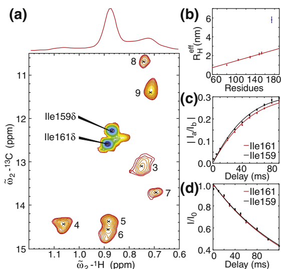
Fig. 1. I159/I161 of \alpha B-crystallin are highly dynamic. (a) Methyl-TROSY spectrum of \text{U-}^2\text{H}_2\text{Ile-}[^{13}\text{CH}_3\text{-}\delta 1]\alpha B-crystallin, 18.8 T, 50 °C, pH 7. A 1D projection of the 2D data set is shown above the spectrum. The nine expected resonances are indicated (there are nine Ile per monomer), with the two especially sharp resonances assigned to positions 159 and 161 highlighted. (b) Hydrodynamic radii of a range of proteins measured using pulsed field gradient NMR. The hydrodynamic radius of a folded protein is expected to scale with the number of residues, N , according to R_H^{\text{eff}} \propto N^{0.23} (continuous line). 38 The value measured for oligomeric \alpha B-crystallin (blue) is 2.16 times larger than expected for a monomer of 175 residues, consistent with a complex composed of approximately 30 subunits. The globular, monomeric proteins used as calibrants were ABP1P-SH3 (80 residues), cytochrome C (104 residues), lysozyme (129 residues), calmodulin (148 residues) and myoglobin (153 residues). (c) Time dependencies of sums ( I_b ) and differences ( I_a ) of magnetization derived from methyl ^1\text{H} single-quantum transitions from which the product S_{\text{axis}}^2\tau_C can be determined. 39 A value of 3.5 ns was obtained for both Ile159 and 161, consistent with their location in an unstructured region. (d) The decay of slowly relaxing proton magnetisation at 30 °C, pH 7, from which the transverse proton relaxation rate, R_2 , can be determined. 40 The relaxation rates for Ile159 and 161 were found to be 6 \text{ s}^{-1} .
