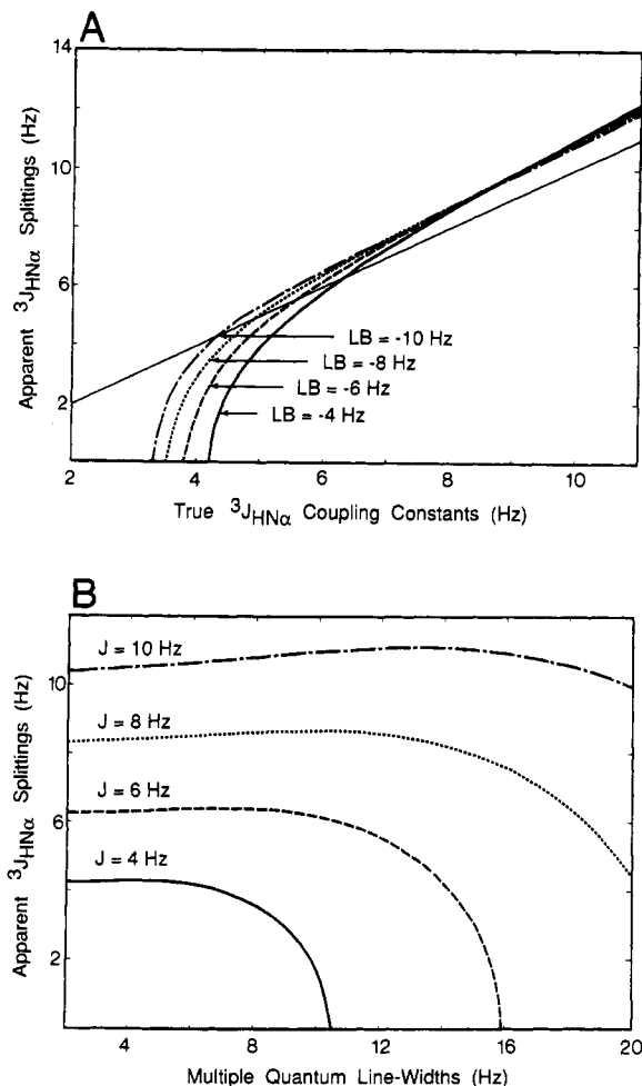
FIGURE 3: (A) Apparent {}^3J_{\text{HN}\alpha} splittings extracted from line shapes simulated by Fourier transformation of the t_1 time domain response, plotted as a function of the true {}^3J_{\text{HN}\alpha} value for different negative line-broadening values (LB) of the Gaussian apodization function of -10 Hz (---), -8 Hz (---), -6 Hz (---), and -4 Hz (—), assuming a multiple quantum line width of 10 Hz. Note that the Gaussian curve used has a maximum at the end of the time domain (i.e., GB = 1). To guide the eye, a straight line given by {}^3J_{\text{HN}\alpha}(\text{apparent}) = {}^3J_{\text{HN}\alpha}(\text{true}) is also drawn. (B) Apparent {}^3J_{\text{HN}\alpha} splittings as a function of multiple quantum line width, for values of the true {}^3J_{\text{HN}\alpha} coupling of 4 Hz (—), 6 Hz (---), 8 Hz (---), and 10 Hz (---), assuming LB = -6 Hz and GB = 1.
