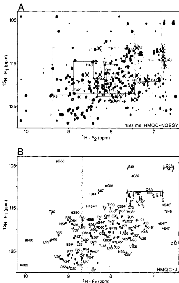
FIGURE 2: ^{15}\text{N} ( F_1 axis)-NH/aromatic ^1\text{H} ( F_2 axis) region of the 150-ms relayed ^{15}\text{N} - ^1\text{H} HMQC-NOESY spectrum (A) and the HMQC- J spectrum (B) of ^{15}\text{N} -labeled reduced recombinant human thioredoxin (30% N-Met/70% N-Val) at 40 °C and pH 5.5. In the HMQC-NOESY spectrum (A) selected ^{15}\text{N}(i) -NH( i+1 ) connectivities from residue Ser-7 to residue Gln-12 and from Phe-41* to Lys-48* are indicated. Peaks with distinguishable chemical shifts between the two forms and arising from the major N-terminal Val species are denoted with an asterisk.
