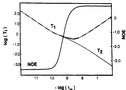
FIGURE 2: Plots of \log(T_1/T_2) and ^1\text{H} – ^{15}\text{N} NOE vs \log(\tau_m) for ^{15}\text{N} relaxed by ^1\text{H} – ^{15}\text{N} dipolar and CSA interactions at a nitrogen frequency of 50.7 MHz. An N–H bond vector tumbling isotropically with S^2 = 1.0 and a bond length of 1.02 Å was assumed. A value of \sigma_{\parallel} - \sigma_{\perp} = -160 ppm was used.
