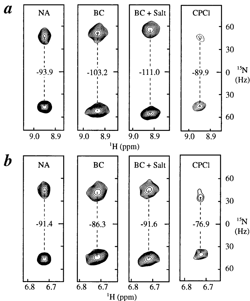
Figure 1. Selected regions of ^{15}\text{N} - ^1\text{H} HN IPAP-HSQC spectra for T4SS in the indicated alignment media for residues (a) Leu39 and (b) Trp126 (where spectra containing upfield and downfield peaks have been superimposed). NA refers to the sample that is not aligned, while brief descriptions of the aligned samples are given in Table 1. The zero point on the vertical scale is centered between the two peaks in the doublet and measured splittings are given for each doublet in Hz. Low peak intensities in the CPCl spectra arise from the low concentration of protein for this particular sample (0.2 mM, as described in Materials and Methods).
